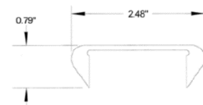
Aluminum Insert
